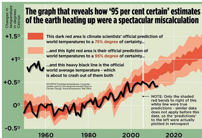
Figure 23: Global Warming.
